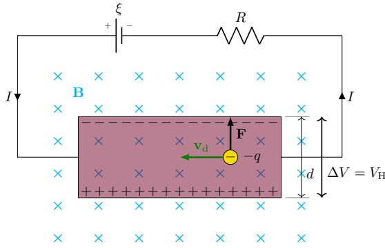
Figure 2: Hall effect when negative charge carriers are flowing through the circuit
